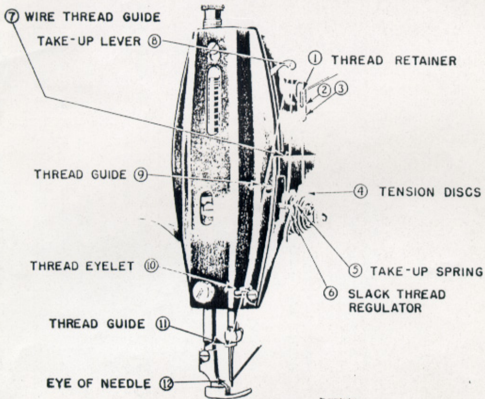
Fig. 3 Upper Threading
